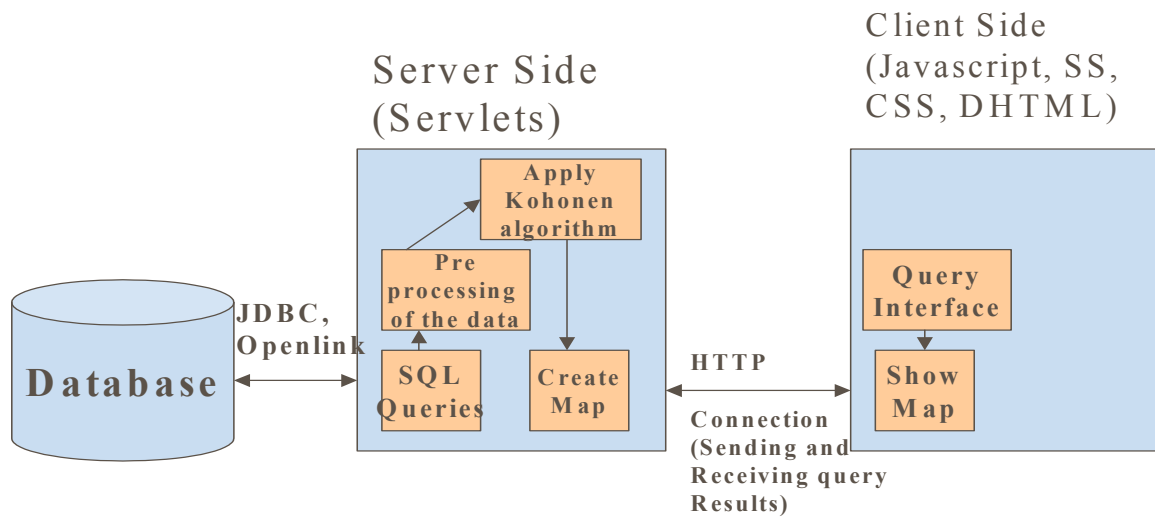
Figure 6. Client-server system design.
