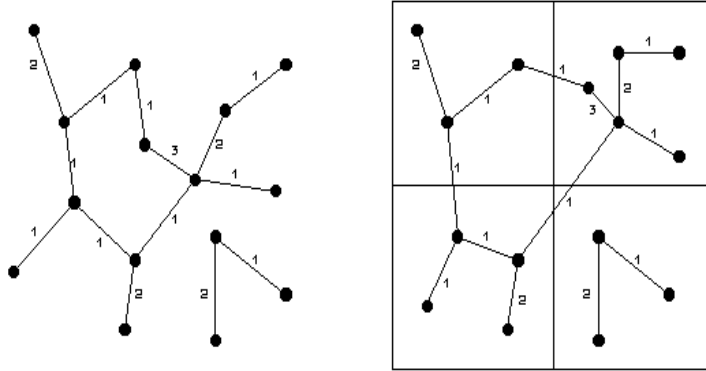
Figure 3. Graph clustering: illustration of the principle used to produce the map shown in Figure 2. Left: graph of objects (author names, articles titles, astronomical objects) with association weights. Right: mapping into a grid of clusters using a homogeneity criterion.
