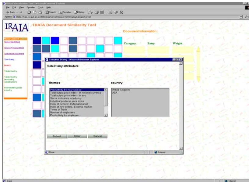
Figure 9. When the user presses “Specialize Document”, the dialog box above appears.
