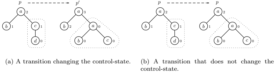
Figure 1: Transitions of a senescent GTRS.
