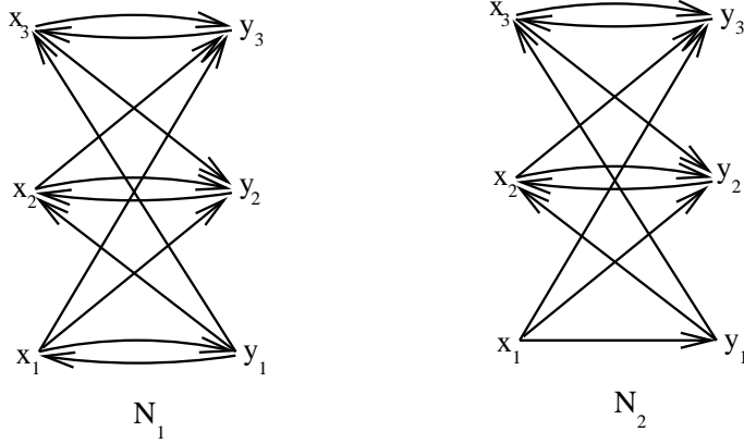
FIG. 1.3. The digraphs N_1 and N_2
