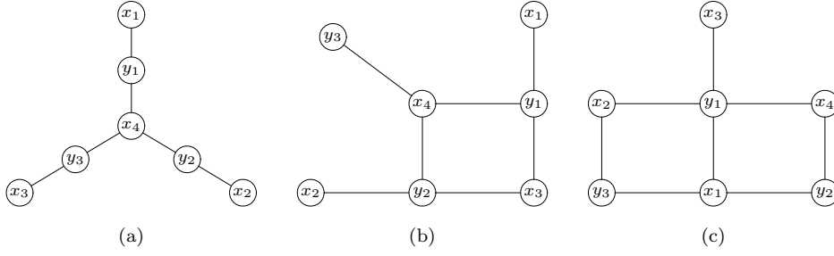
FIG. 1.1. A bipartite claw (a), a bipartite net (b) and a bipartite tent (c).
