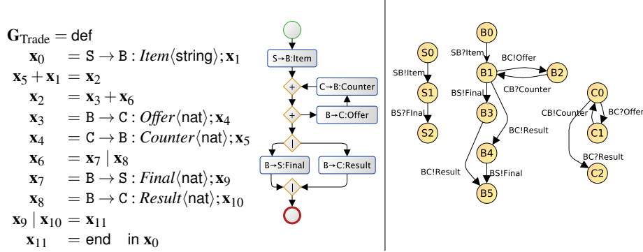
Fig. 1. Trade Example: Global Type and CFMSM
