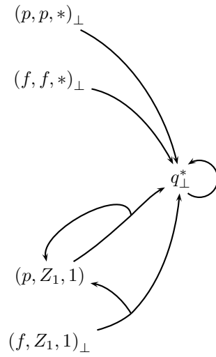
Figure 11: The result of the first greatest fixed point calculation with some states hidden for presentational purposes.
