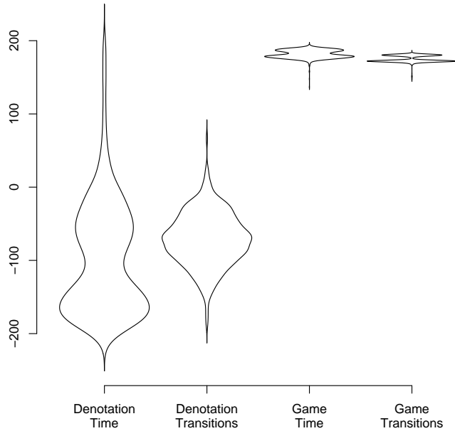
Figure 15: The percentage difference in the performance of the two algorithms for computing the denotation of a formula and the winning region of a game, both in terms of time and maximum number of transitions. A negative value indicates that the denotation approach was superior, and a positive value favours the game approach. The label indicates whether the problem instance was a modal \mu -calculus formula, or a parity game. Each violin plot compares both approaches for the stated problem and performance metric.
