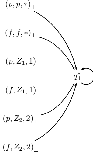
Figure 6: The automaton after introducing initial valuations of Z_1 and Z_2 .
