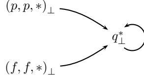
Figure 5: The automaton giving initial valuations of p and f .
