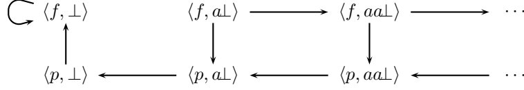
Figure 1: The configuration graph of an example pushdown system.
