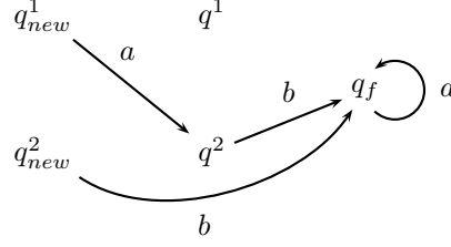
Figure 3: A_{eg} updated by the rules p^1 a \rightarrow p^2 \varepsilon and p^2 b \rightarrow p^2 ba .
