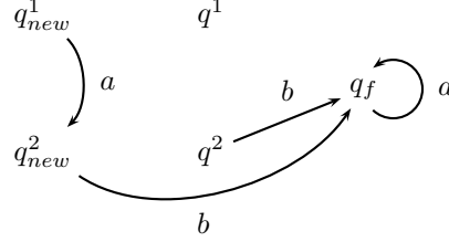
Figure 4: The result of projecting the automaton in Figure 3.
