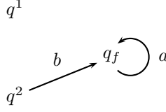
Figure 2: The automaton A_{eg} accepting \langle p^2, ba^* \rangle .
