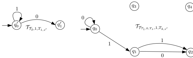
Fig. 4. \mathcal{T}_{\mathcal{T}_2, 1, T_{1,z'}} and \mathcal{T}_{\mathcal{T}_{\mathcal{T}_1, 0, T_z}, 1, T_{2,z'}}
