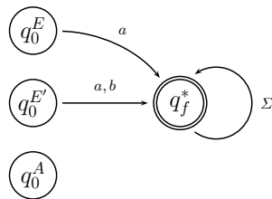
Fig. 6. The automaton accepting the winning region of Éloïse.
