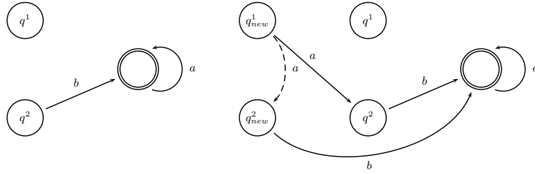
Fig. 1. (i) On the left, A_{eg} accepting \langle p^2, ba^* \rangle ; and, (ii) on the right, A_{eg} updated by the rules p^1 a \rightarrow p^2 \varepsilon and p^2 a \rightarrow p^2 ba . The dashed line is the result of projection.
