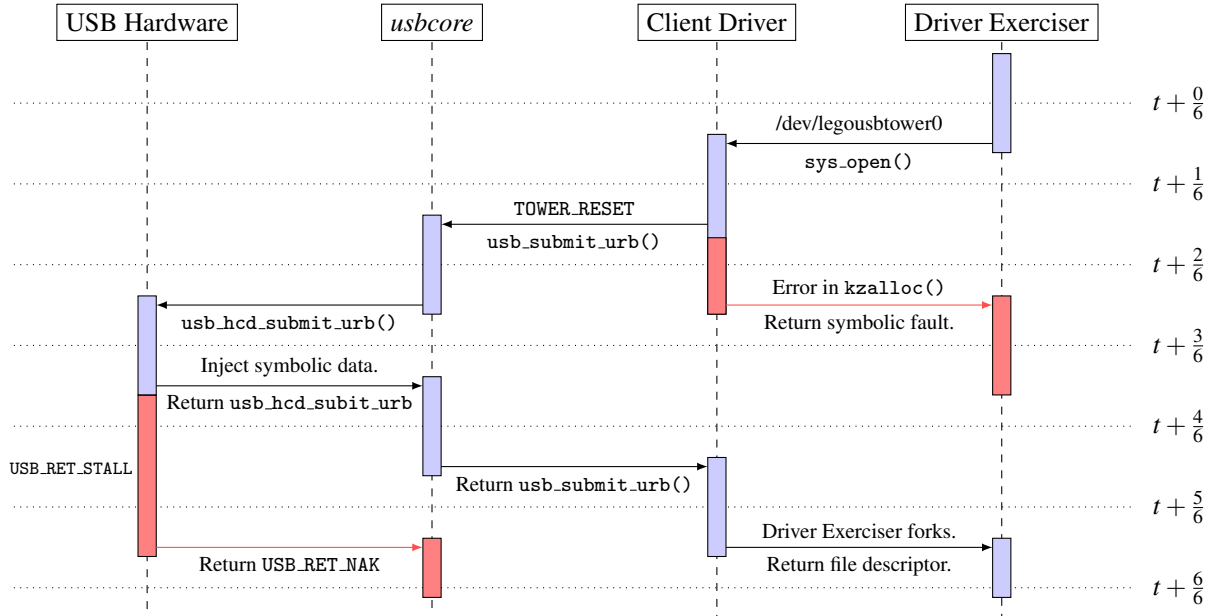
Figure 2: Example of flows for viable code paths from the driver exerciser through the Linux USB stack. The diagram shows fault injection and fork points for the legousbtower client driver.
